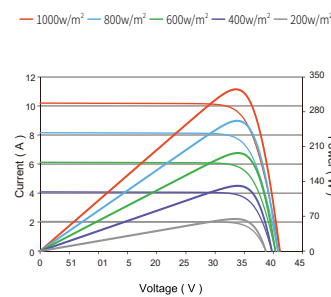
Current-Voltage & Power-Voltage Curves (325W)
