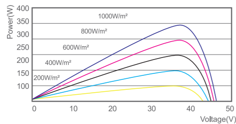
PV Curve (340W)
