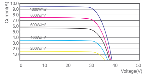
IV Curve (340W)
